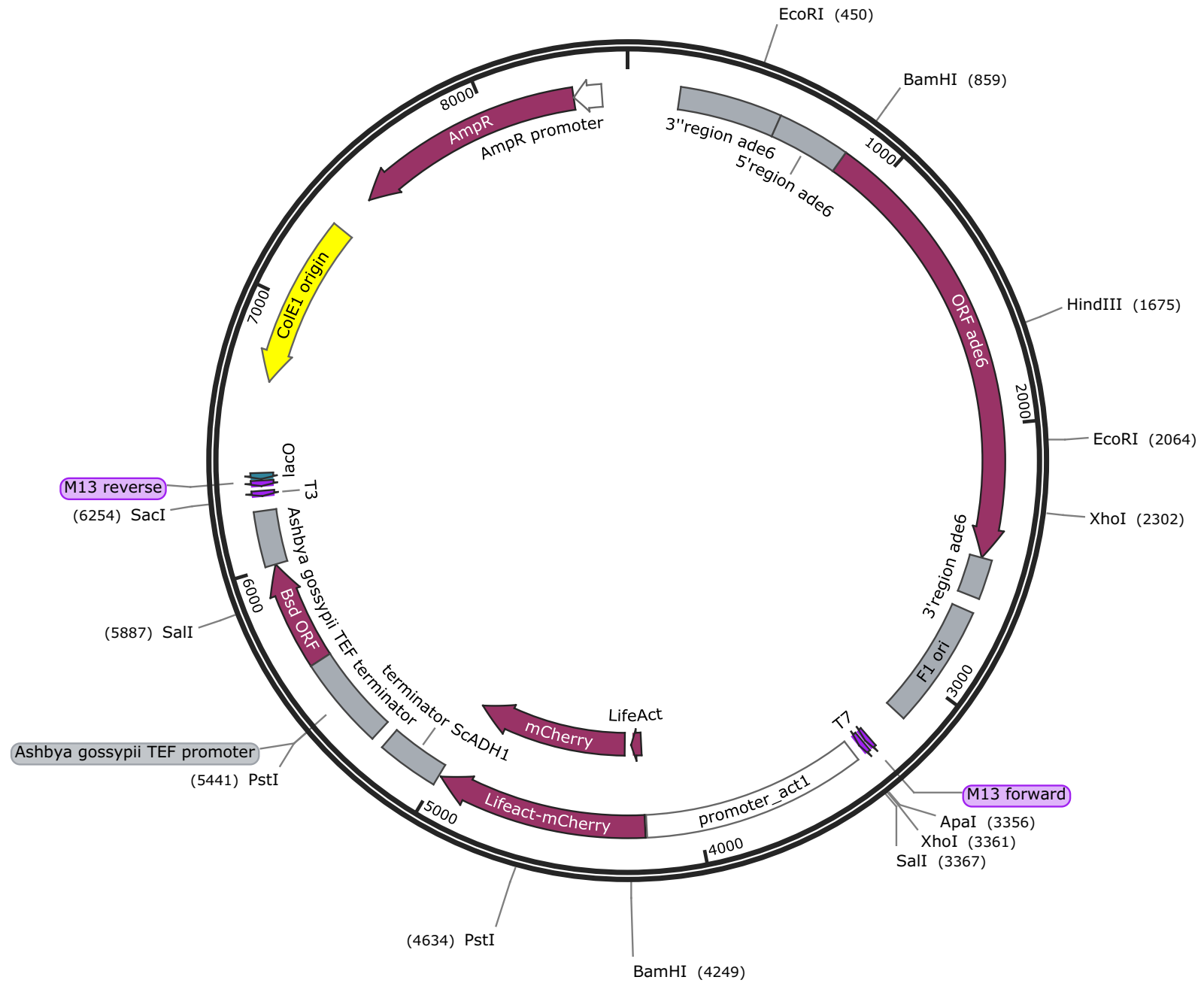
pAV0783 pAde6PmeI-pact1-LifeAct-mCherry-termScADH1-bsdMX 8528 bp
